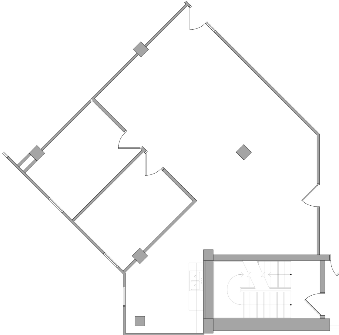
1 FLOOR PLAN A-1 1/8" = 1'-0"
